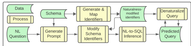
Figure 6: Experiment setup workflow from NL question and schema as input to predicted query as output.
