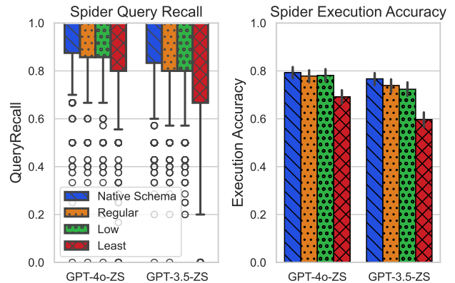
Figure 13: QueryRecall and Execution Accuracy differences over the Spider [58] dev set modified using SNAILS renaming artifacts.
