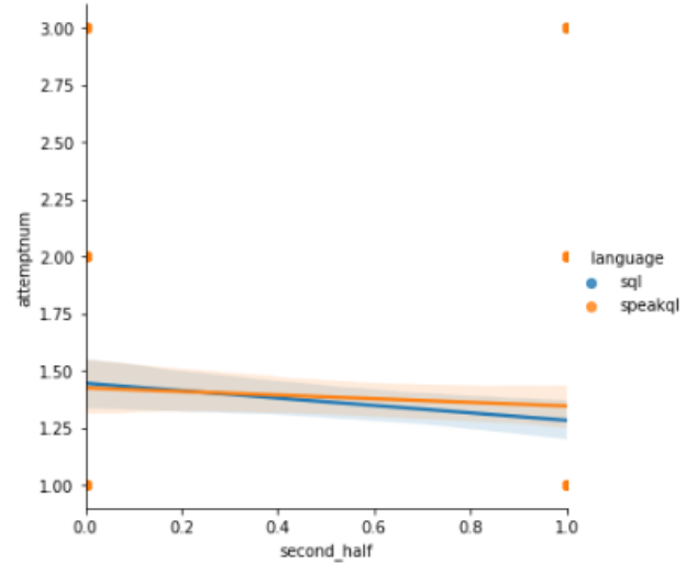
Figure 25: Learning Effect - SpeakQL Attempt Number Performance Improvement
