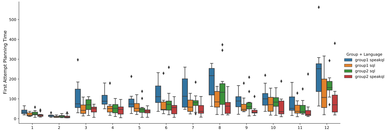
Figure 28: Dialect performance measured by first attempt planning time and separated by group. Group 1: SpeakQL-first, Group 2: SQL-first
