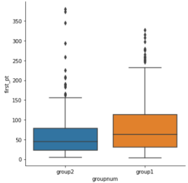
Figure 24: Imbalance Between SpeakQL->SQL (Group 1) and SQL->SpeakQL (Group 2) first planning time performance. Group 1 median: 62.0; Group 2 median: 44.5; Mann-Whitney U Test P Value: 0.00007
