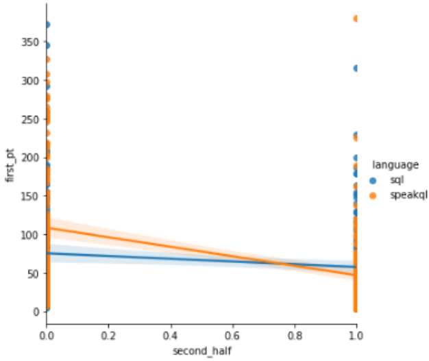
Figure 23: Learning Effect - SpeakQL Planning Time Performance Improvement
