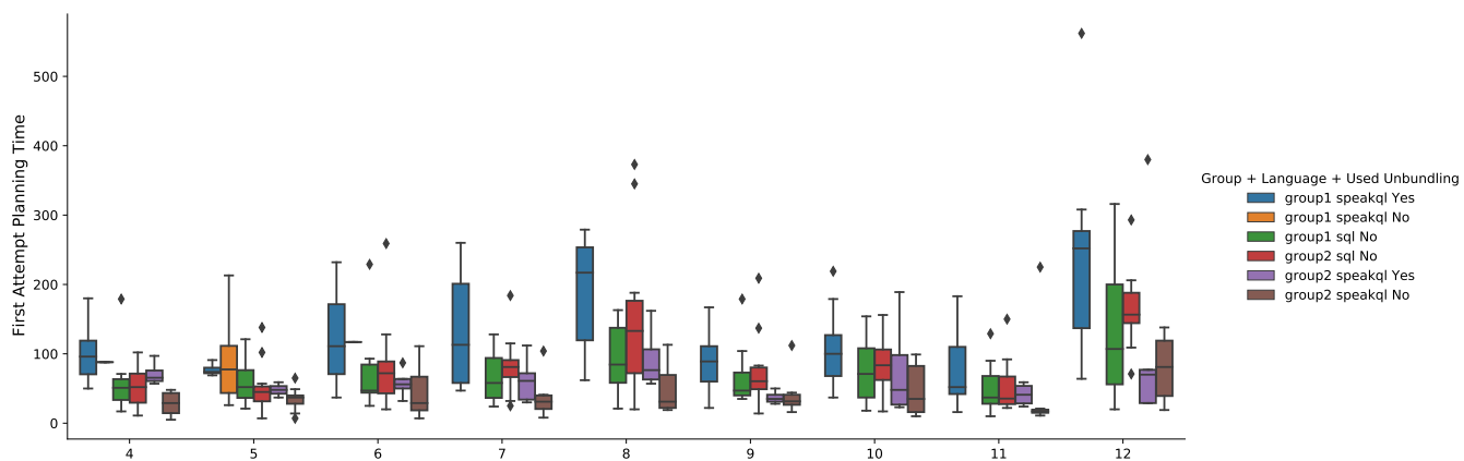
Figure 29: Dialect performance measured by first attempt planning time and separated by group and unbundling usage. Group 1: SpeakQL-first, Group 2: SQL-first
