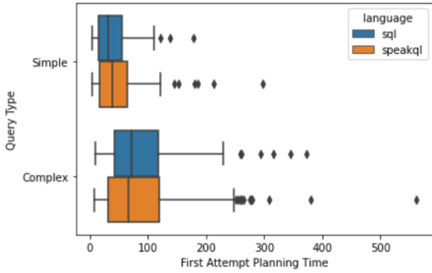
Figure 22: Simple and Complex Query Planning Time
