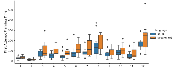
(b) First half - Planning Time, First Attempts, By Individual Query
