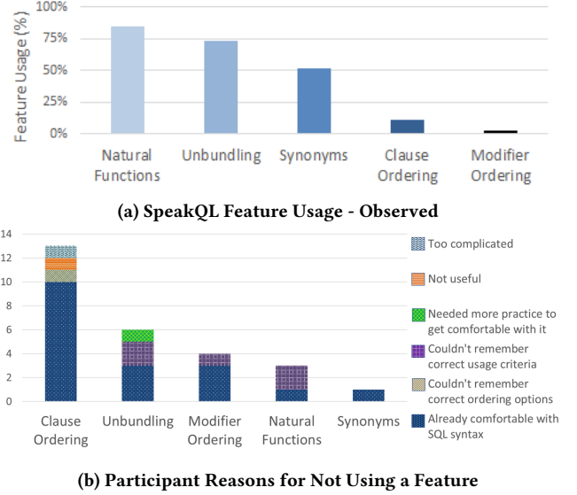
Figure 7: Feature Usage Observations and Avoidance Reasons
