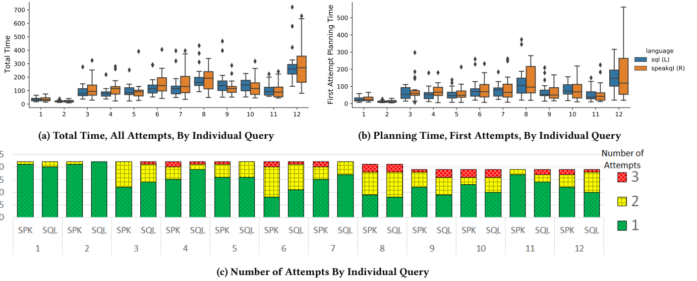
Figure 6: Quantitative results from the user study.
