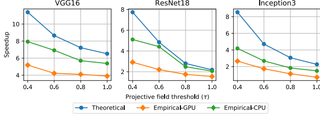
Figure 12: Speedups with incremental inference combined with only projective field thresholding.
